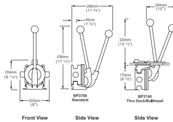
Gusher 10 Mk3 Standard BP3708
