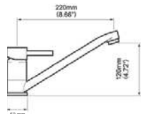
Lever Galley Chrome Faucet TT1111
