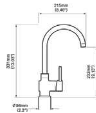
Swan Neck Galley Chrome Faucet TT1211
