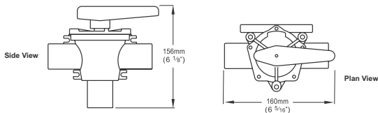
DV5606 For dimensions see page 40 to 42
